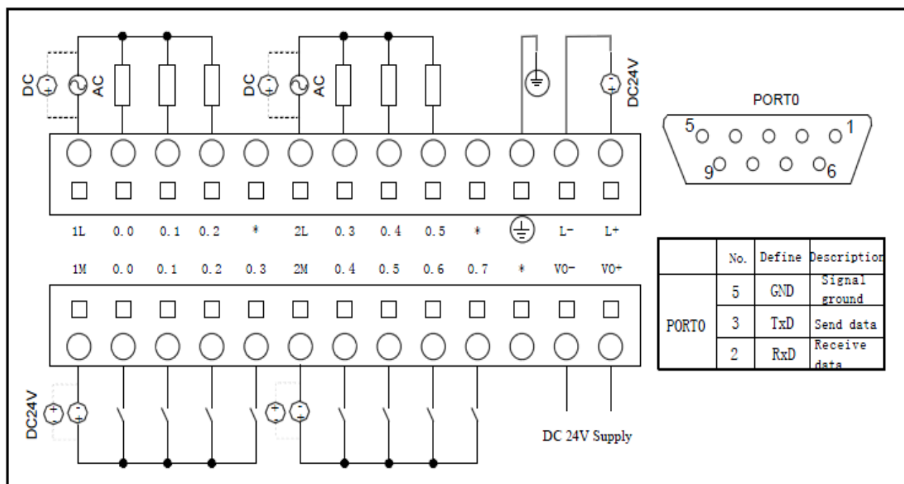
Diagram 2-5 Wiring Diagram of Kinco-K504-14DR
